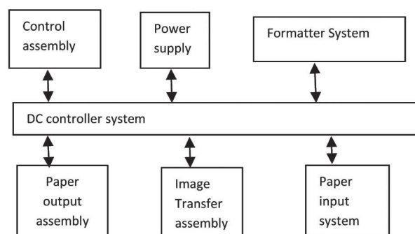
Fig.11 Simplified Block Diagram of printer
