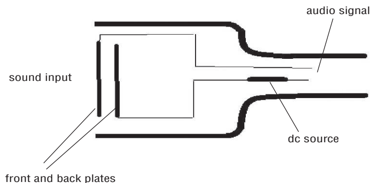
Fig.3 Capacitor microphone
