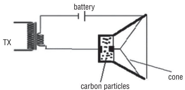
Fig.1 Carbon microphone
