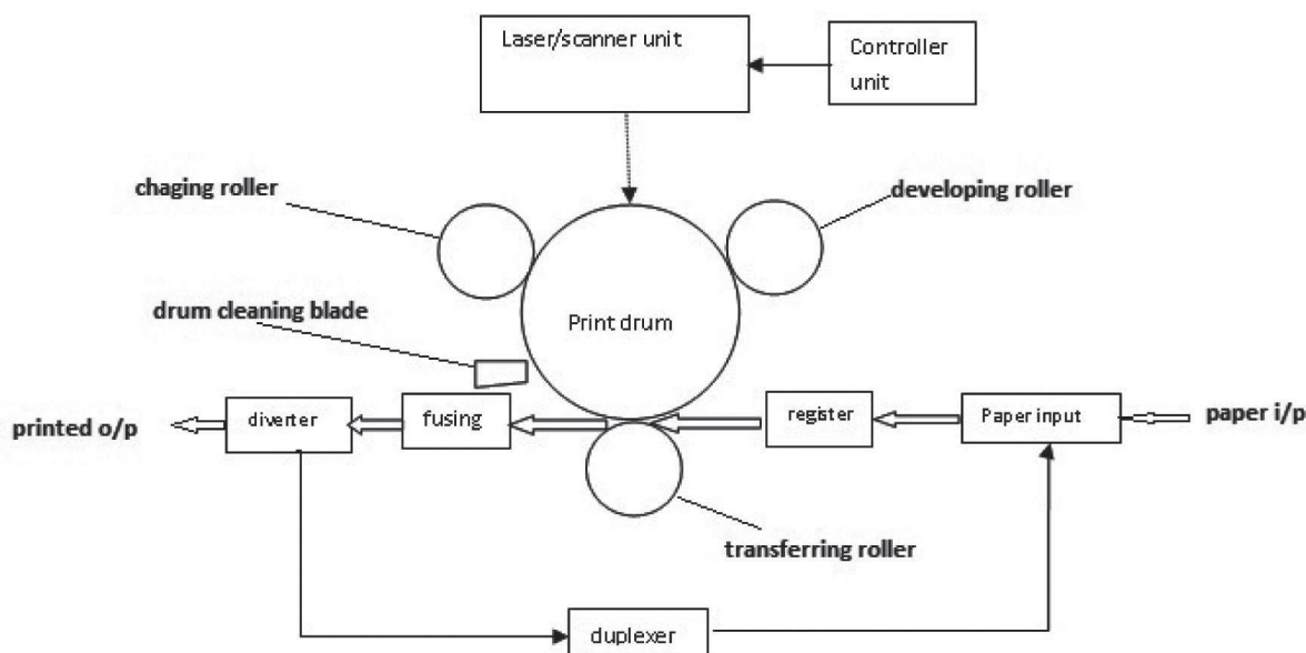
Fig.12 Image Formation Block Diagram
