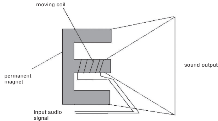
Fig.9 Moving coil loudspeaker
