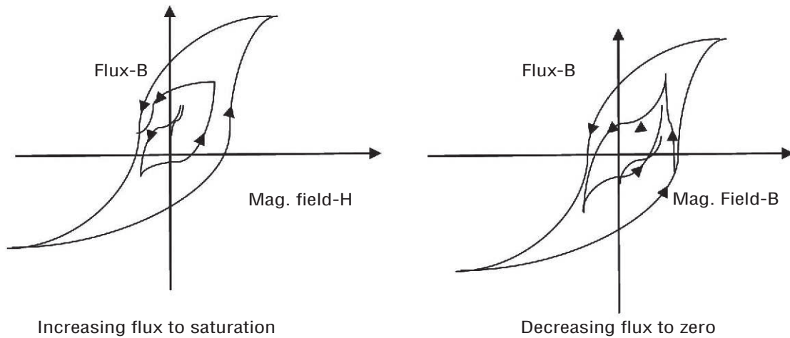
Fig.8 Erasing process
