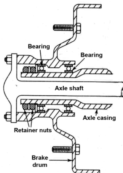
Fig. 4.2.12 Fully-floating Rear Axle
