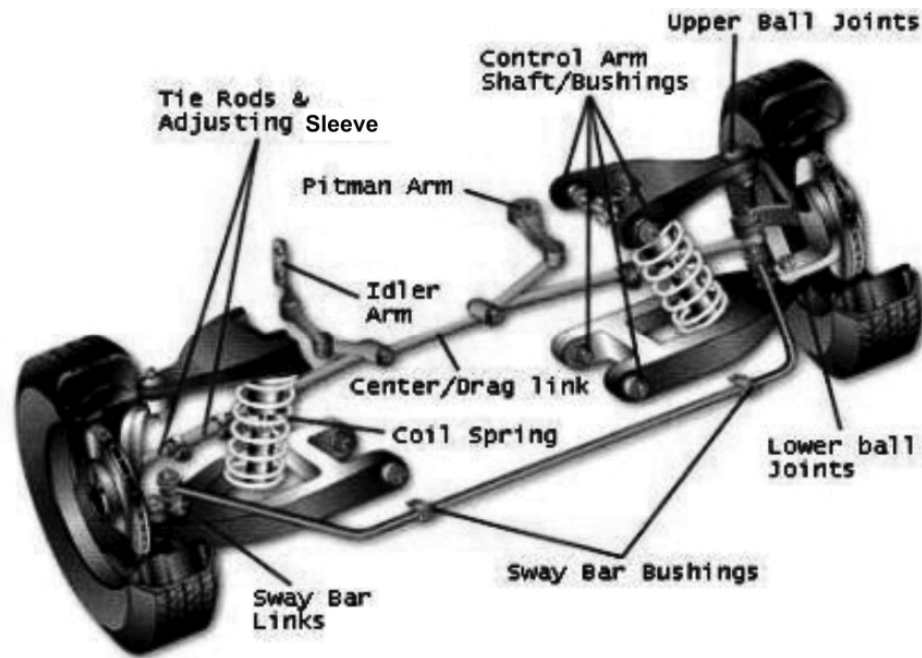
Fig. 3.3 Independent Suspension System
