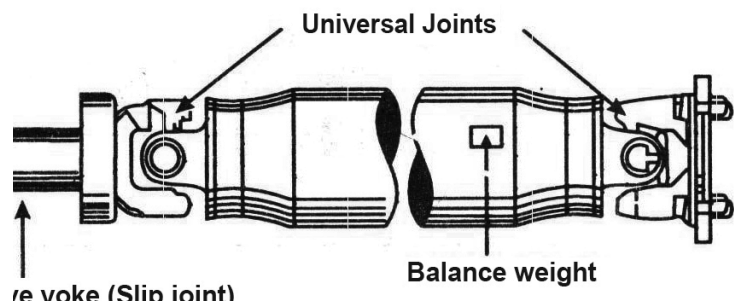
Fig. 4.1.1 Propeller Shaft Assembly
