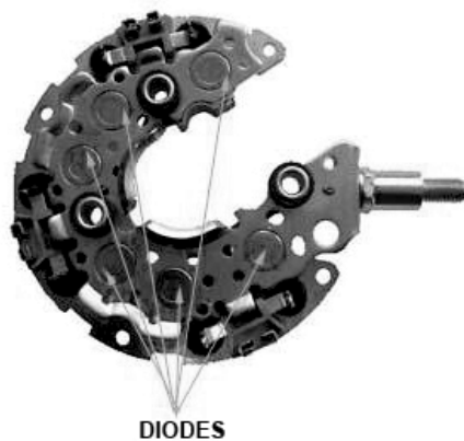
Fig. 5.15 Rectifier Assembly of Alternator
