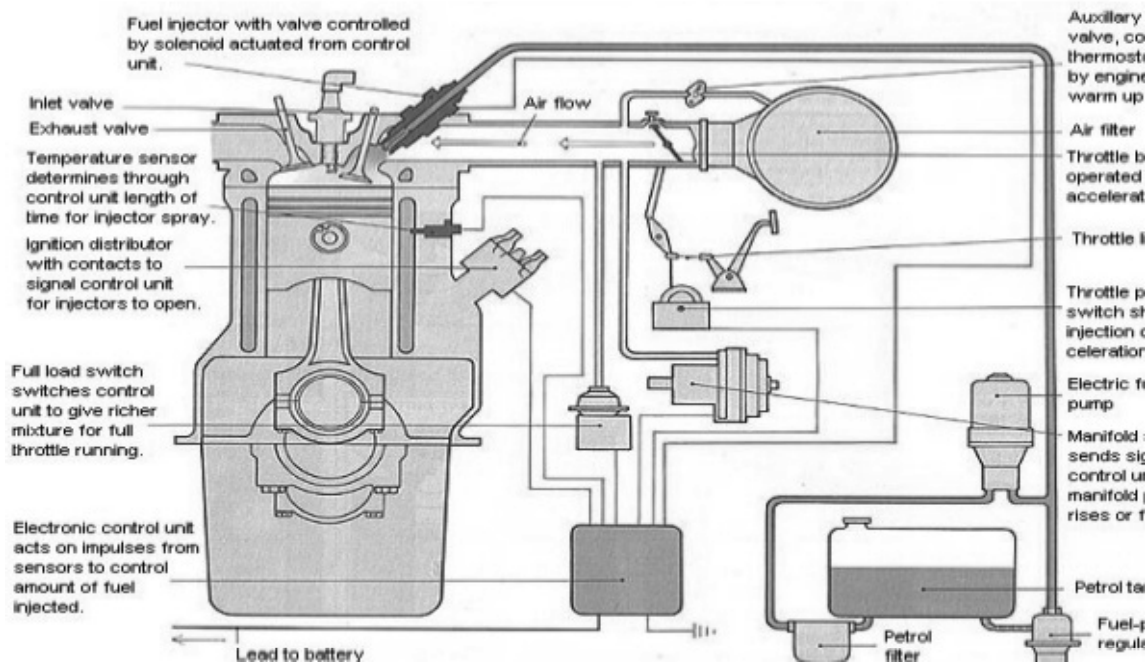
Fig. 5.29: Electronic Fuel Injection System
