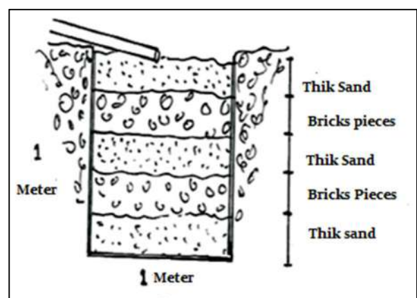
Fig 67 - Soak pit
