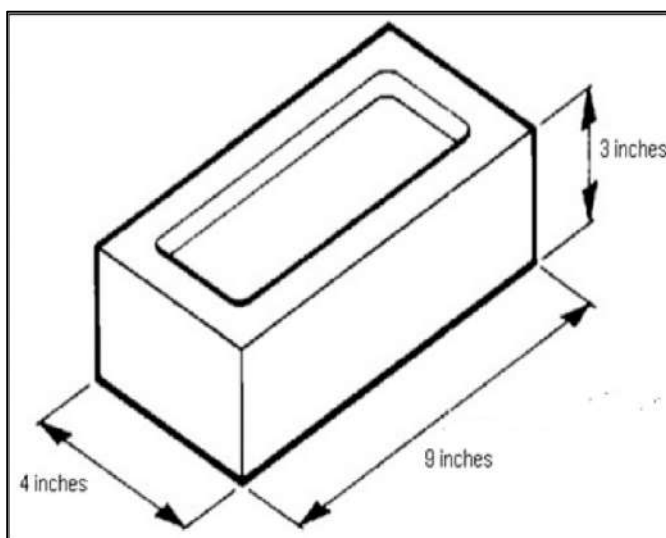
Fig 52 - Bricks
