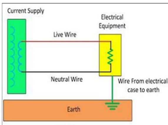
Fig 47 - Earthing
