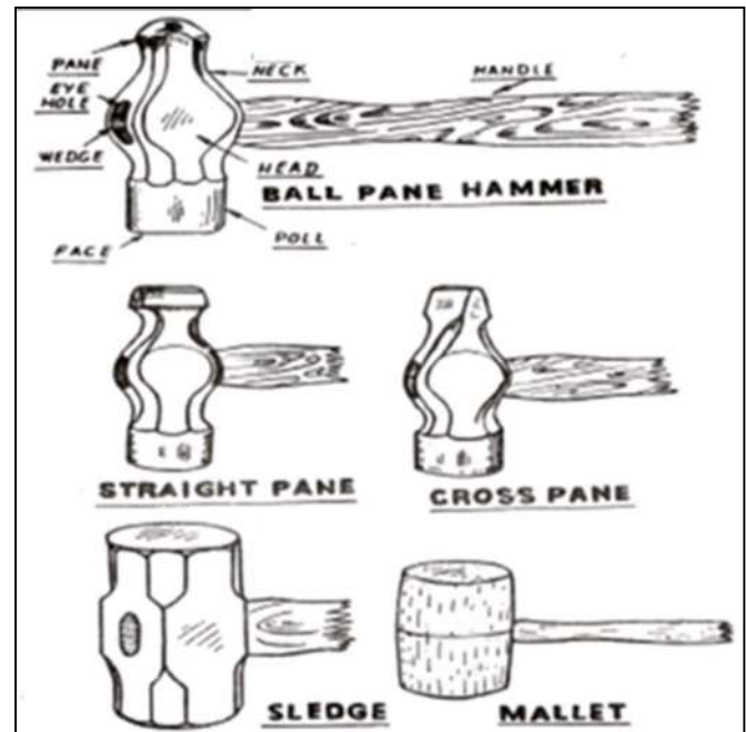
Fig 2 - Hammer
