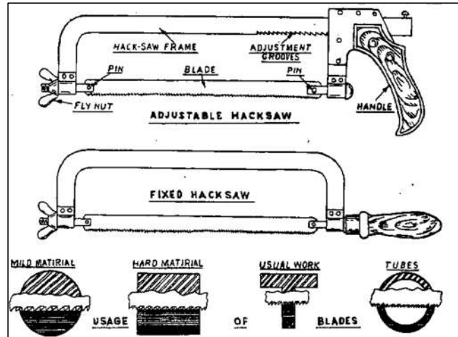
Fig 5- Hacksaw
