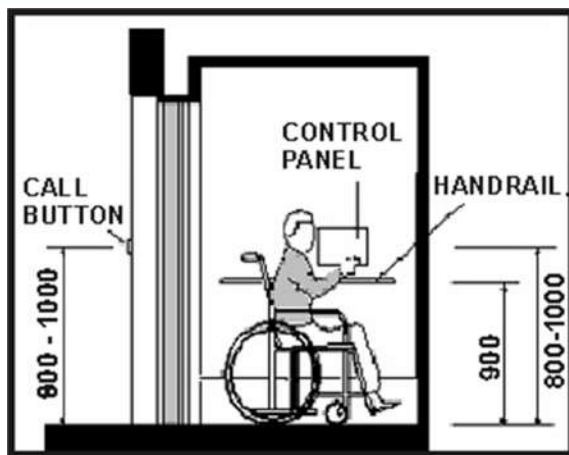
Figure 5.47 Standards for lifts door and control panel with Braille
